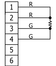
ELECTRICAL CONNECTIONS
