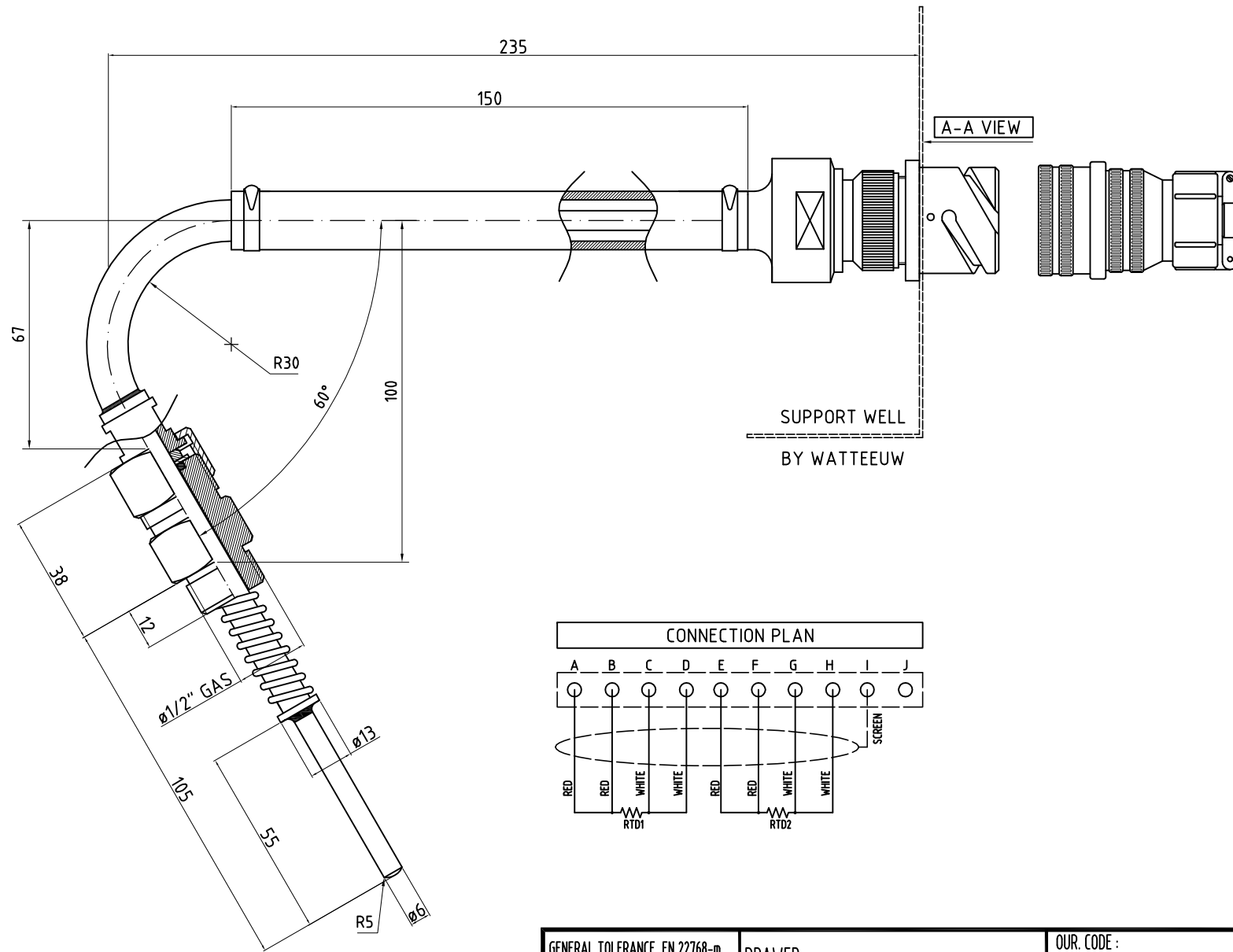
SECTION QUADRANT OF THE CONNECTOR
