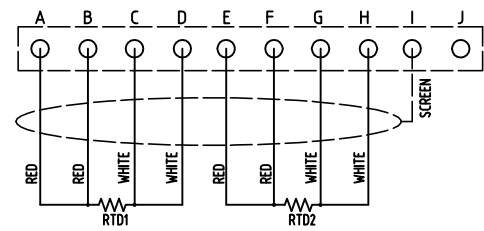
CONNECTION PLAN
